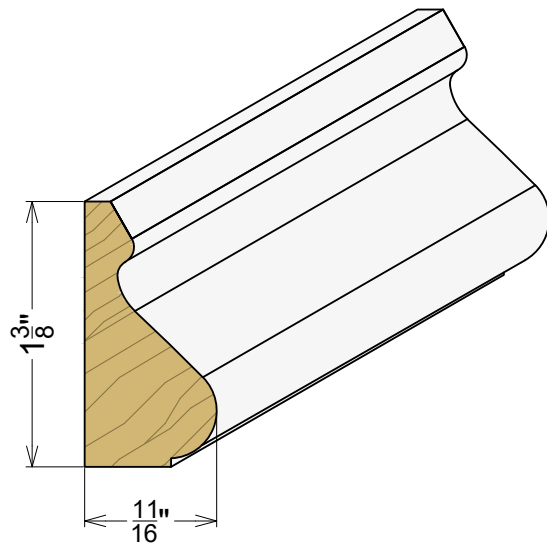
AP 1004 11/16" x 1-3/8"
