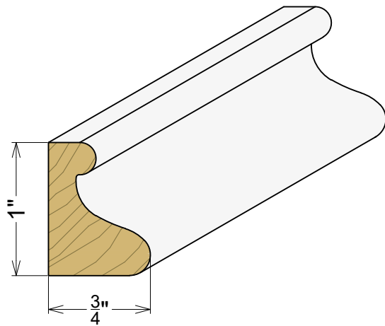
AP 1018 3/4" x 1"
