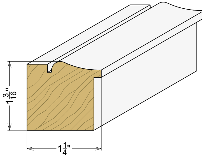
AP 1020 1-3/16" x 1-1/4"
