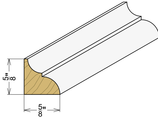
AP 1024 5/8" x 5/8"
