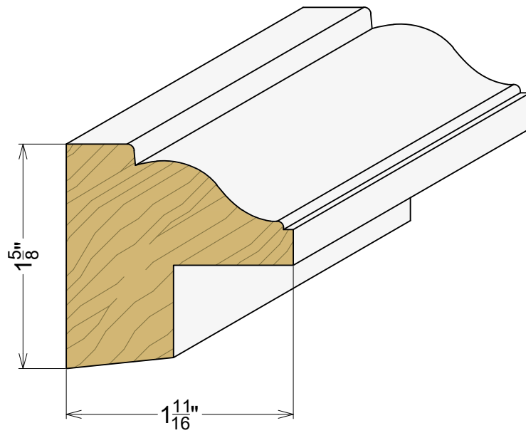
AP 1040 1-5/8" x 1-11/16"
