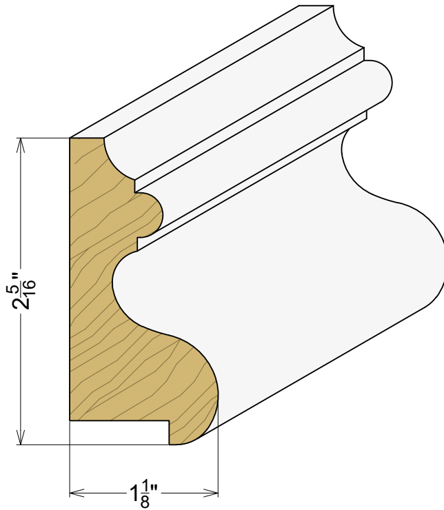
AP 1046 1-1/8" x 2-5/16"
