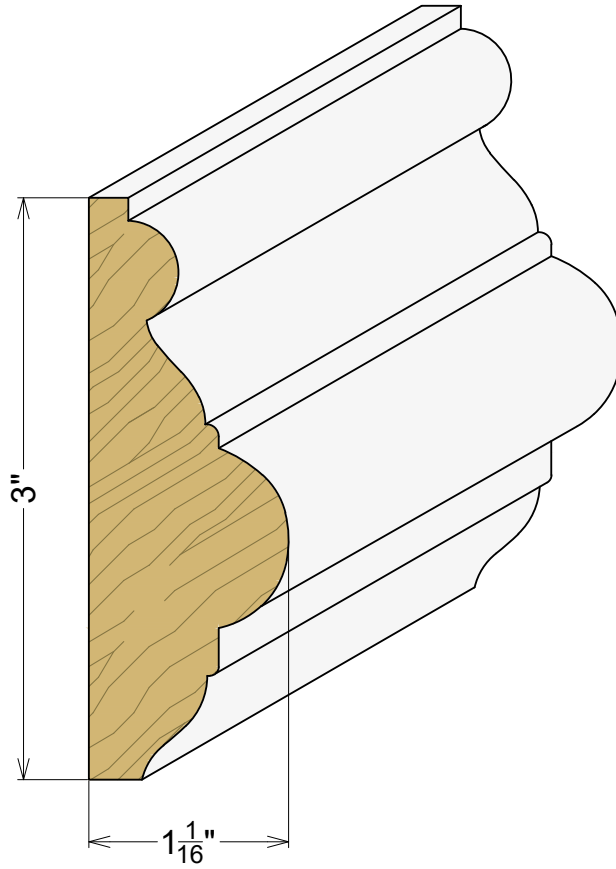
AP 1059 1-1/16" x 3"
