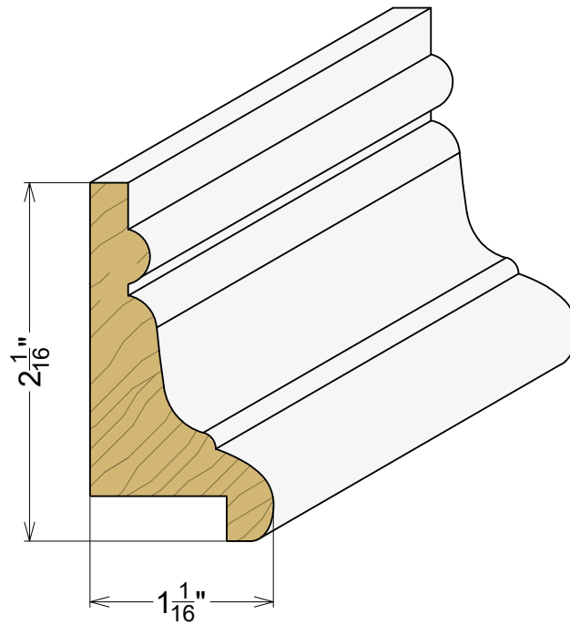
AP 1070 1-1/16" x 2-1/16"
