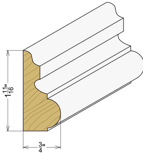
AP 1083 3/4" x 1-11/16"
