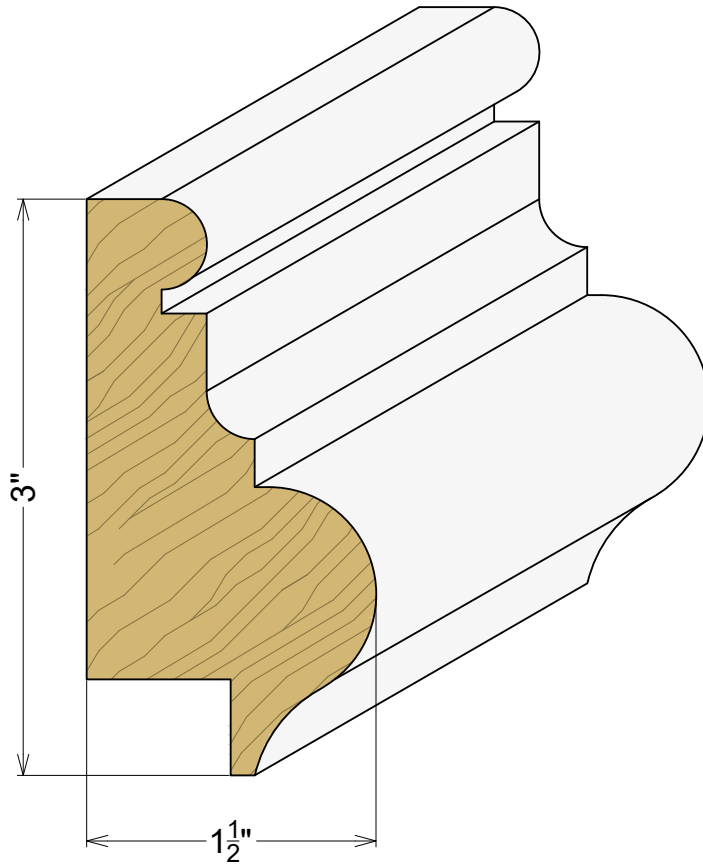
AP 1098 1-1/2" x 3"
