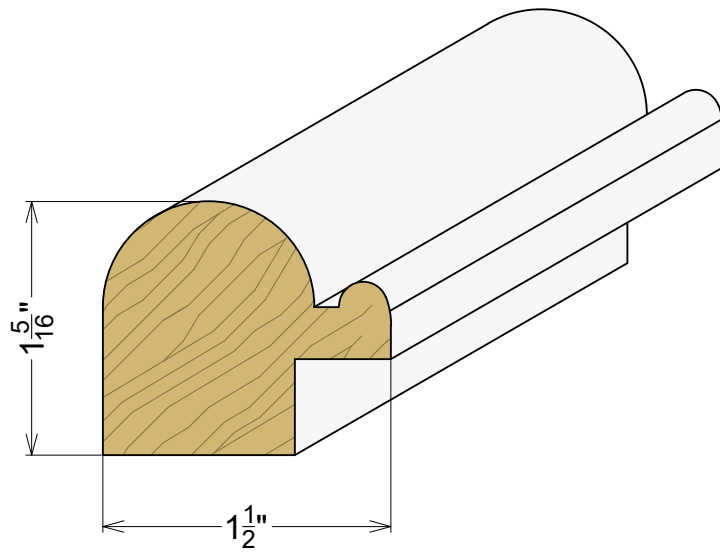
AP 1100 1-5/16" x 1-1/2"
