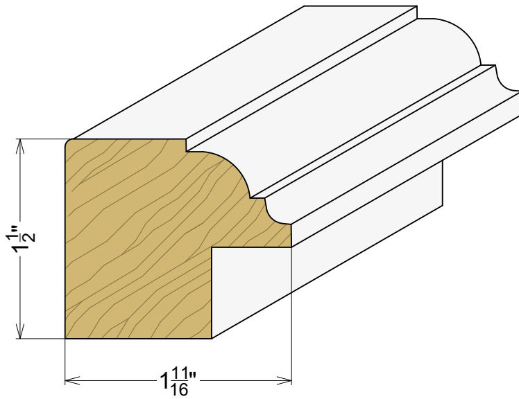
AP 1101 1-11/16" x 1-1/2"
