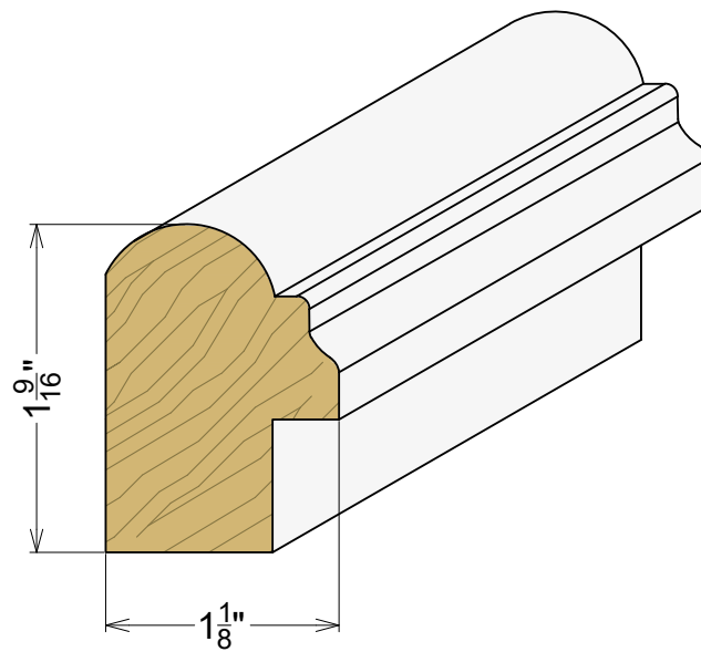
AP 1104 1-1/8" x 1-9/16"
