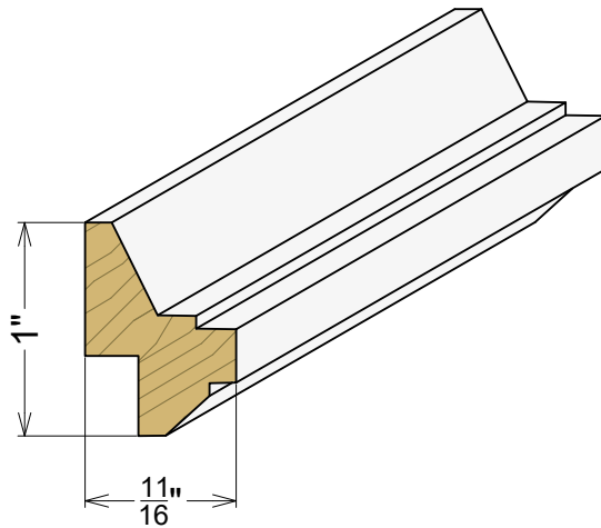
AP 1105 11/16" x 1"
