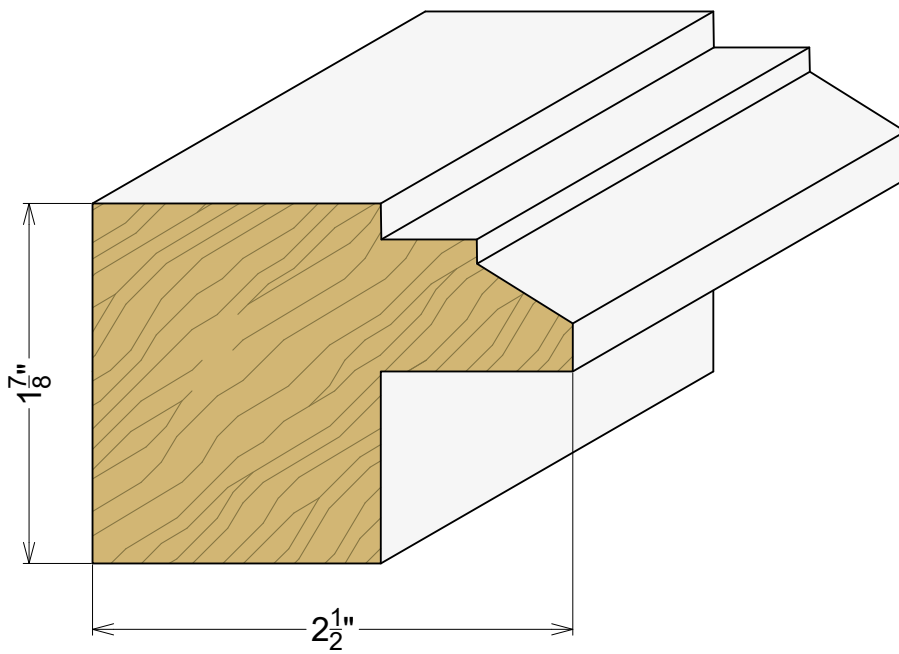
AP 1106 1-7/8" x 2-1/2"
