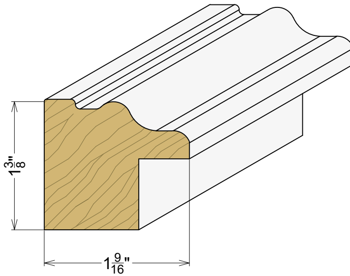
AP 1110 1-3/8" x 1-9/16"
