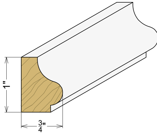
AP 1119 3/4" x 1"
