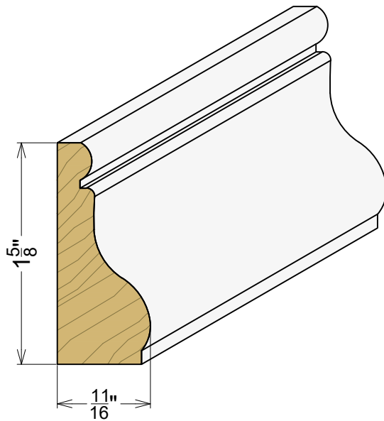
AP 1142 11/16" x 1-5/8"
