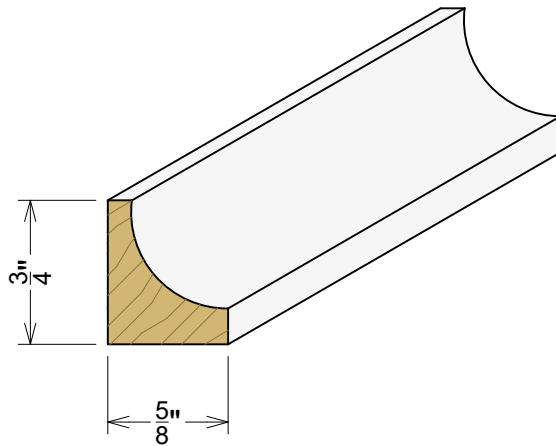
AP 1154 5/8"x 3/4"
