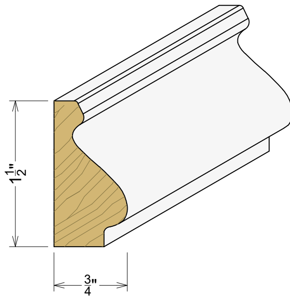
AP 1155 3/4"x 1 1/2"
