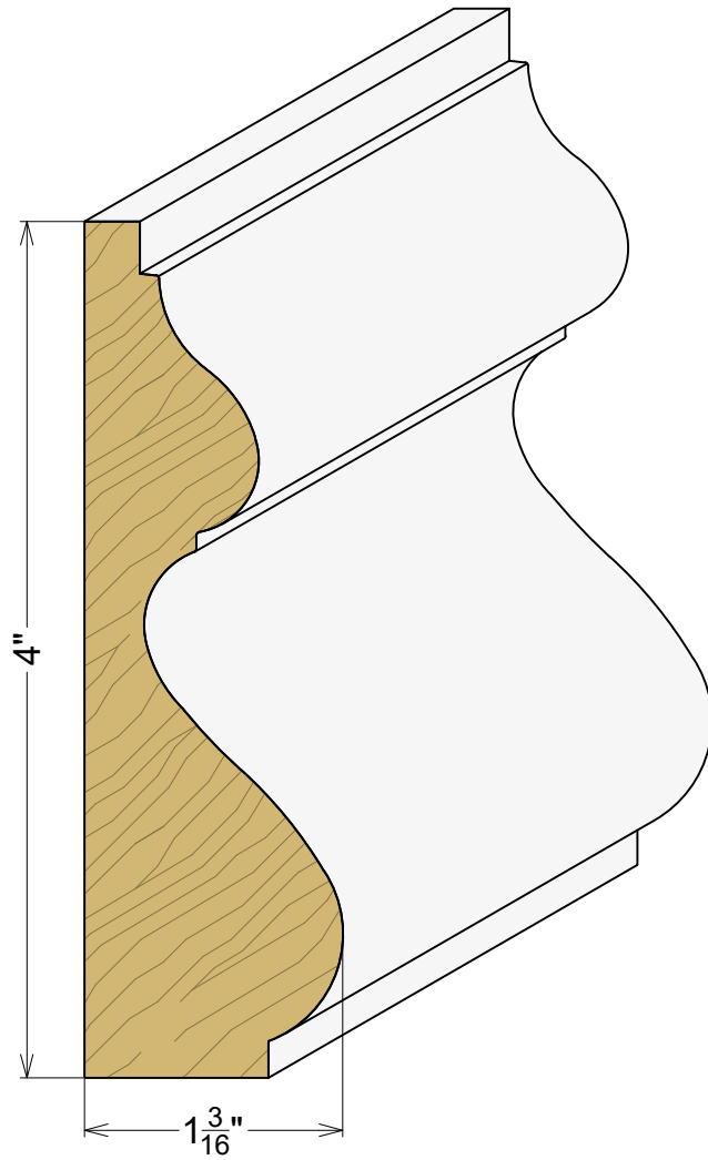
AP 2596 1-3/16" x 4"
