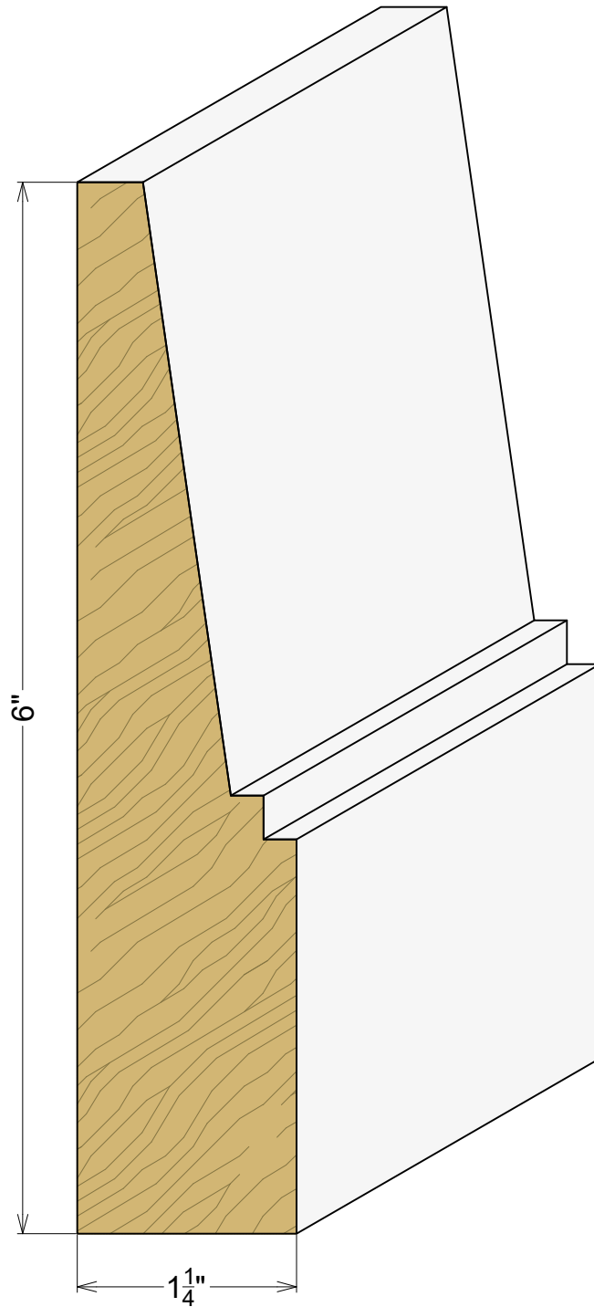
AP 2601 1-1/4" x 6"
