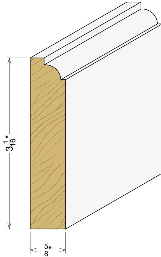
AP 2653 5/8"x 3 1/16"
