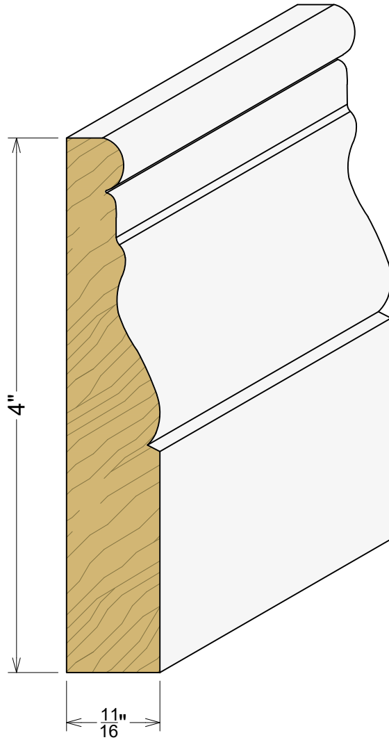
AP 2662 11/16"x 4"
