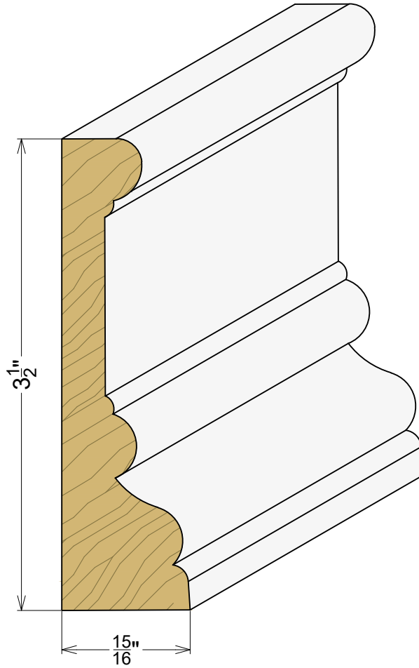
AP 2043 15/16" x 3-1/2"
