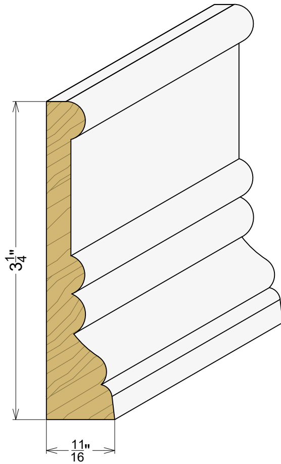
AP 2045 11/16" x 3-1/4"
