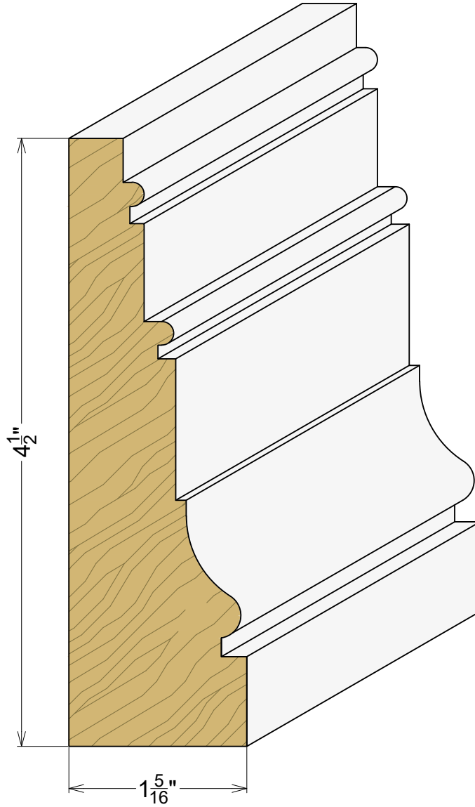
AP 2058 1-5/16" x 4-1/2"
