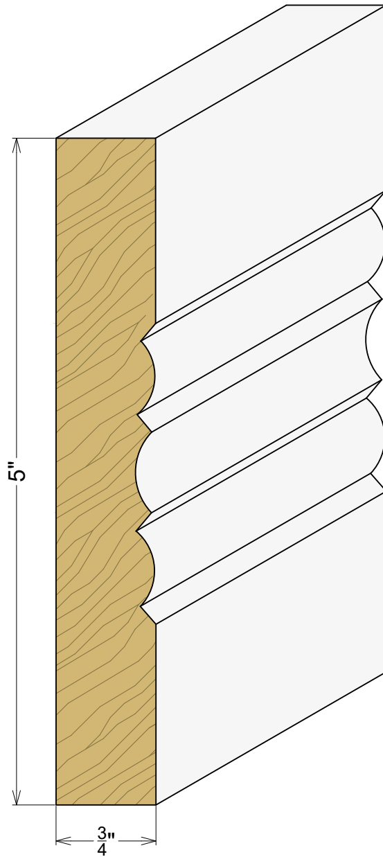
AP 2063 3/4" x 5"
