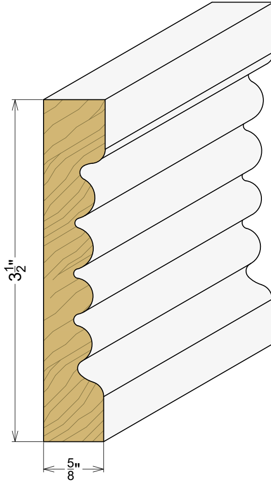
AP 2070 5/8" x 3-1/2"
