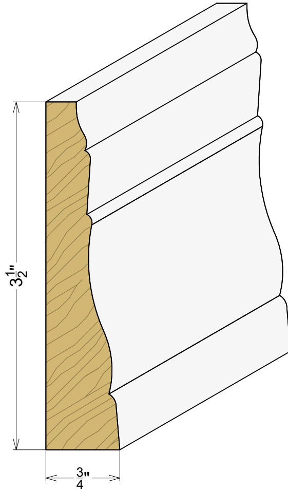
AP 2086 3/4" x 3-1/2"
