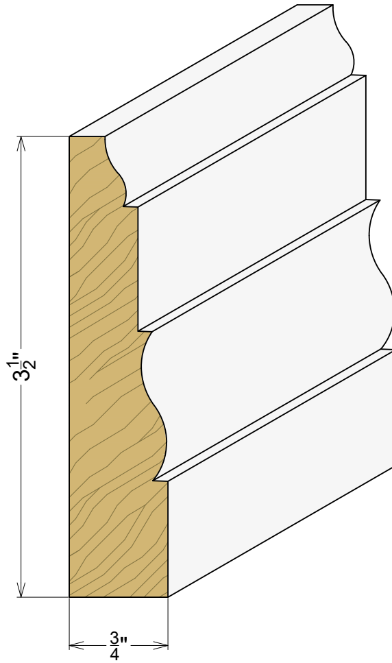
AP 2107 3/4" x 3-1/2"
