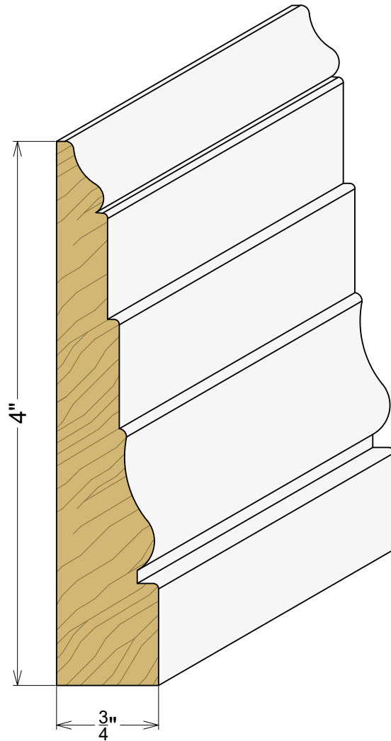
AP 2110 3/4" x 4"
