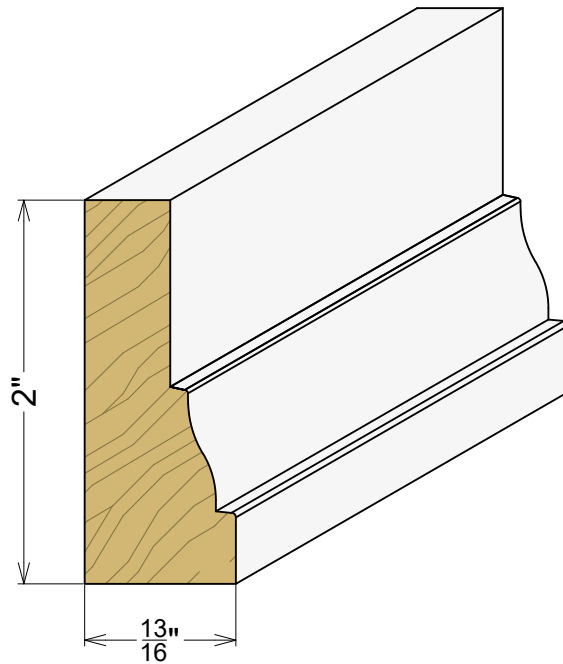
AP 2118 13/16" x 2"
