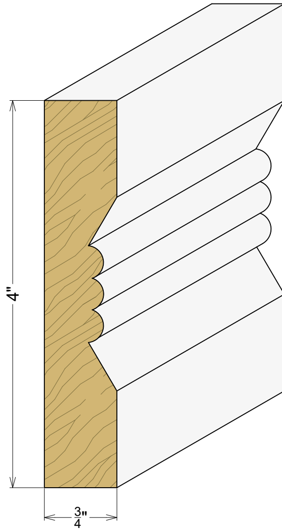
AP 2136 3/4" x 4"
