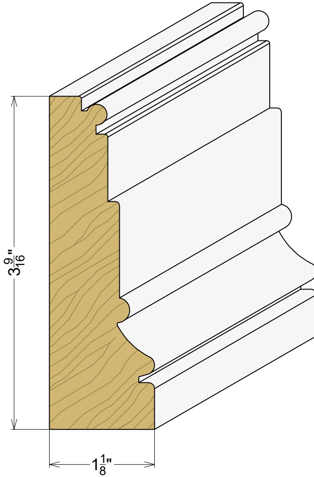
AP 2141 1-1/8" x 3-9/16"
