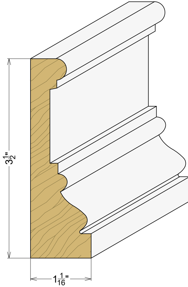
AP 2143 1-1/16" x 3-1/2"
