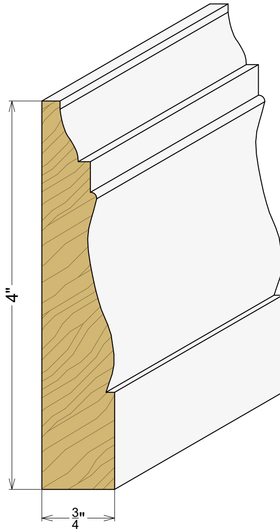
AP 2145 3/4" x 4"
