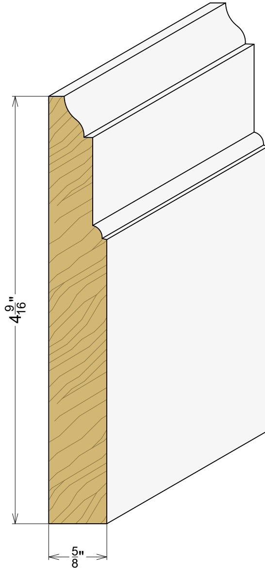
AP 2150 5/8" x 4-9/16"
