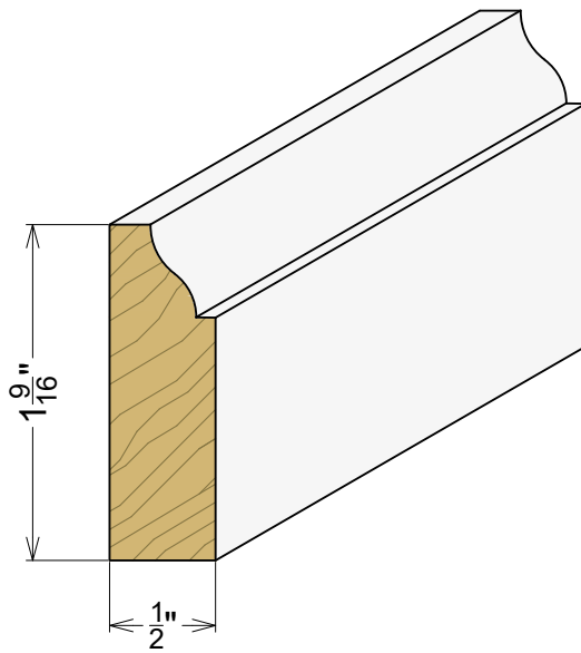
AP 2151 1/2" x 1-9/16"
