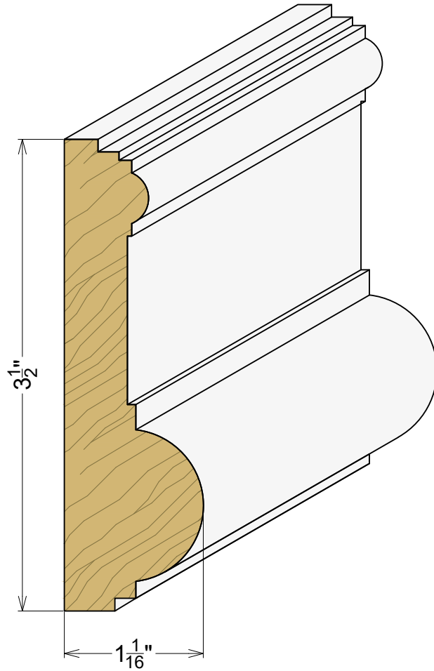
AP 2165 1-1/16" x 3-1/2"
