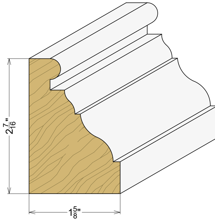
AP 2174 1-5/8" x 2-7/16"
