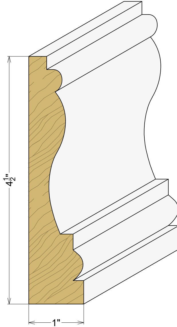
AP 2177 1" x 4-1/2"
