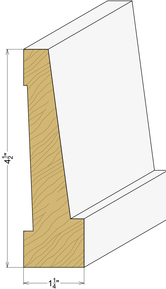
AP 2184 1-1/4" x 4-1/2"
