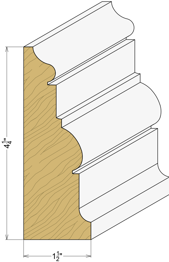
AP 2195 1-1/2" x 4-1/4"
