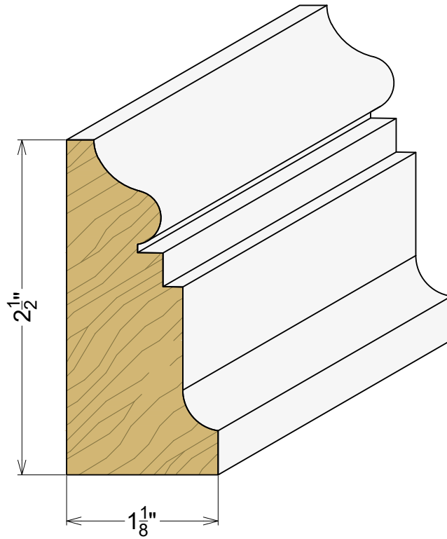
AP 2196 1-1/8" x 2-1/2"
