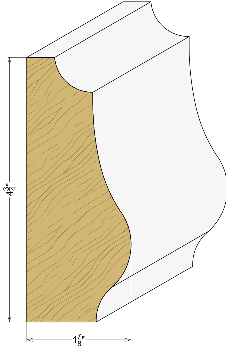
AP 2222 1-7/8" x 4-3/4"
