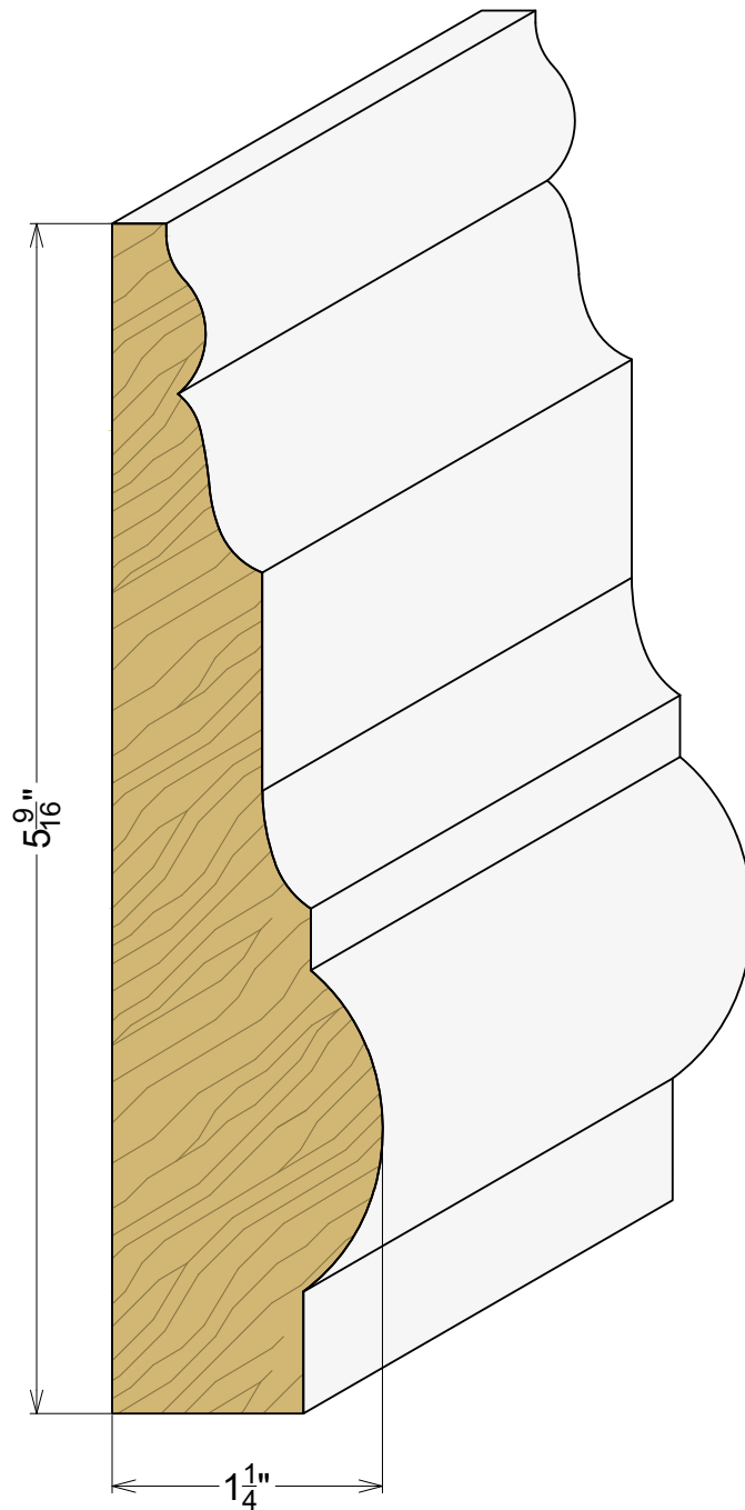
AP 2226 1-1/4" x 5-9/16"
