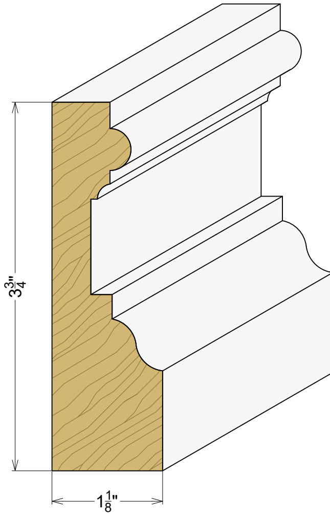
AP 2237 1-1/8" x 3-3/4"
