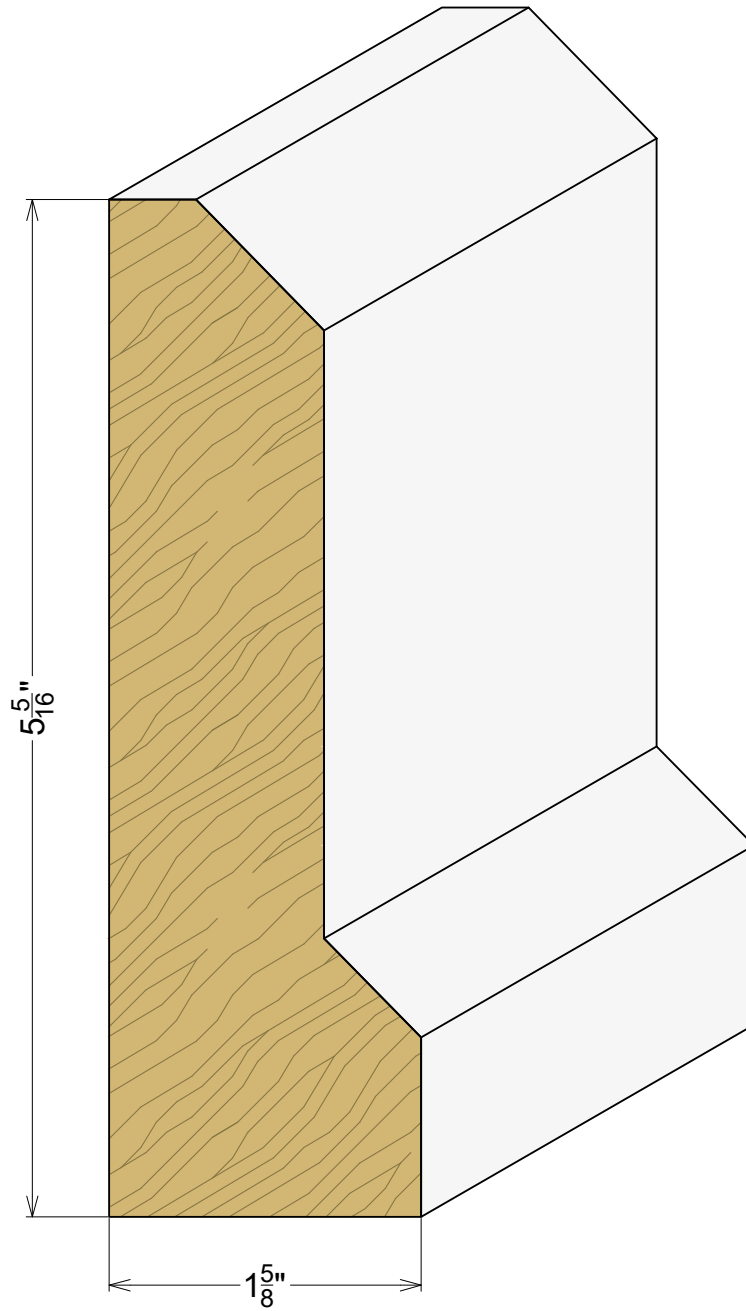
AP 2238 1-5/8" x 5-5/16" Plinth Block
