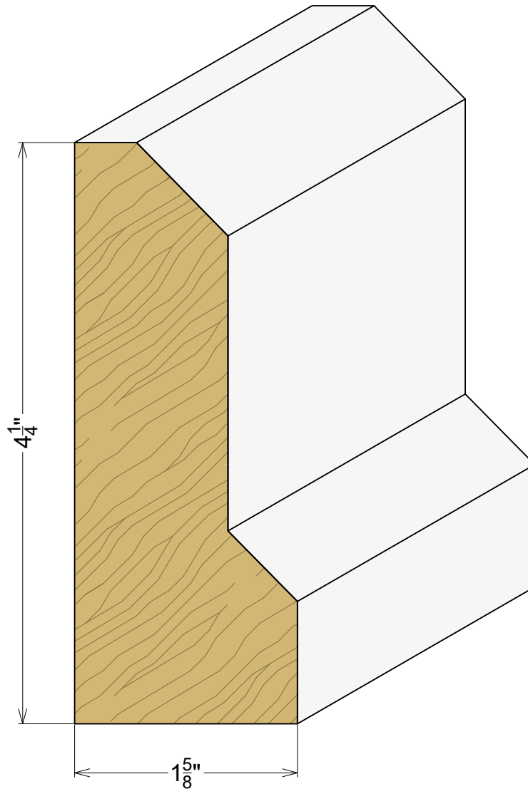
AP 2239 1-5/8" x 4-1/4" Plinth Block
